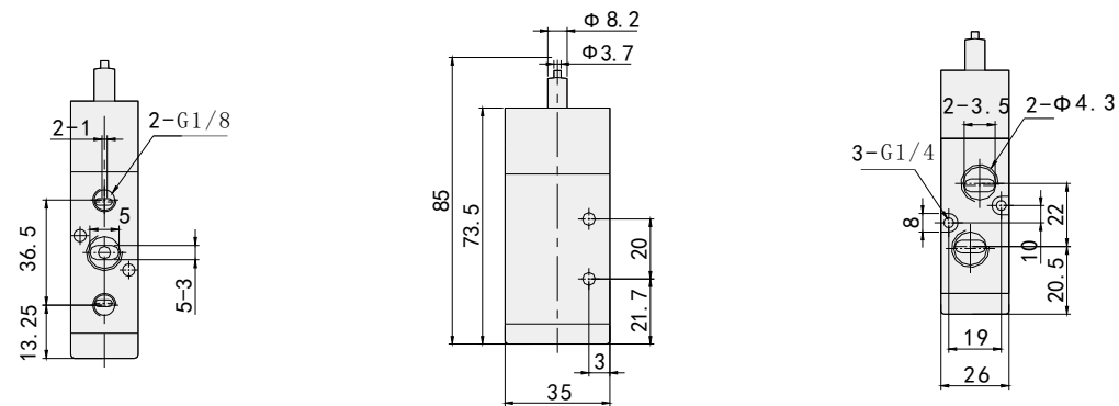
M522 Series
